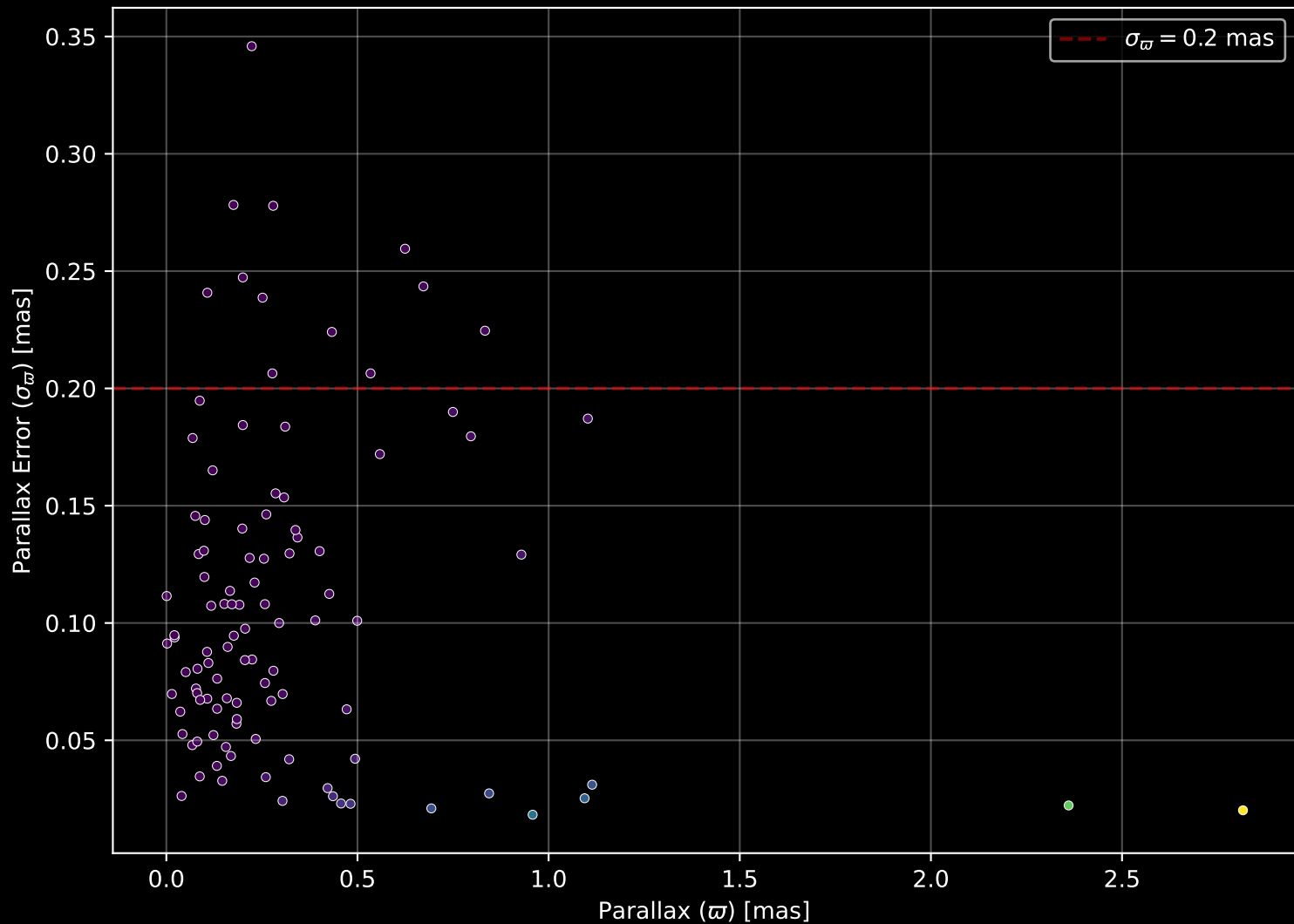
APOGEE DR17 Field: [004+02-O] Parallax Quality (n= 104)
