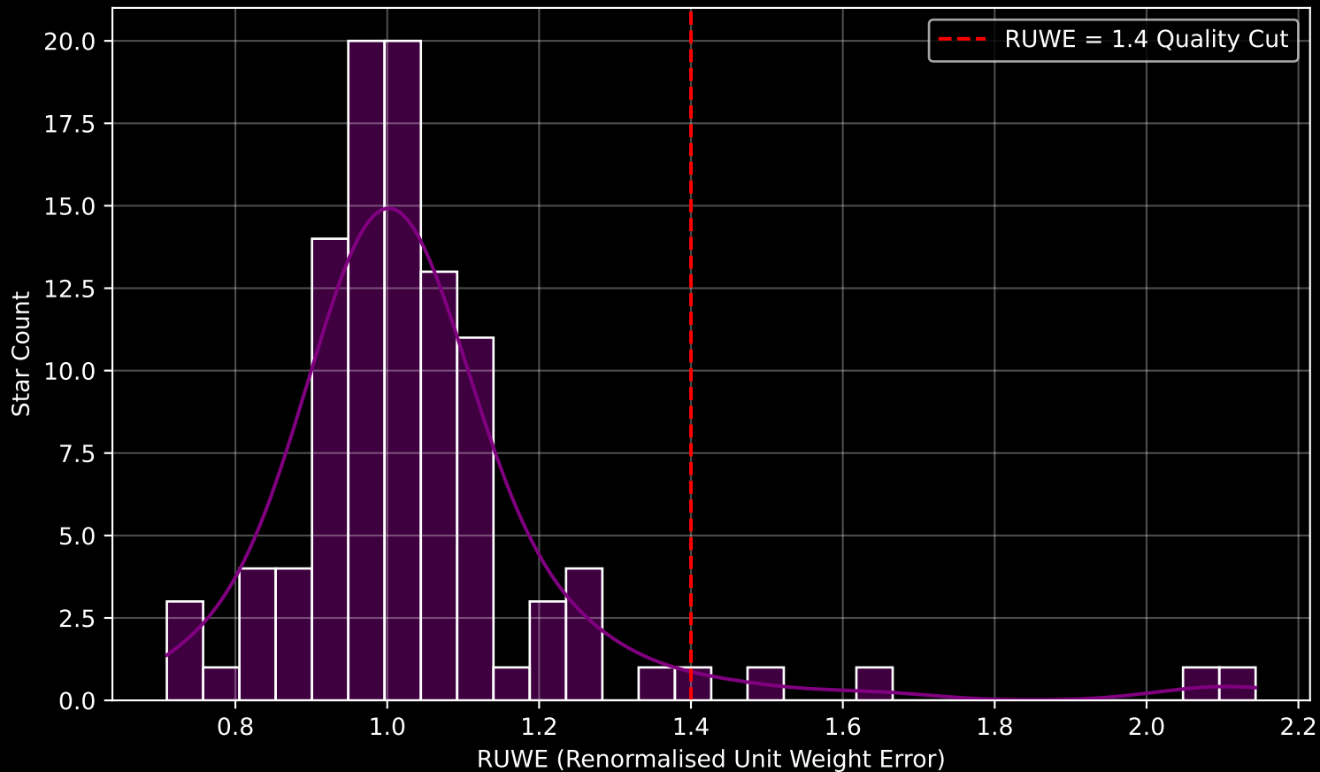
GAPOGEE DR17 Field [004+02-O] RUWE Distribution (n= 104)
