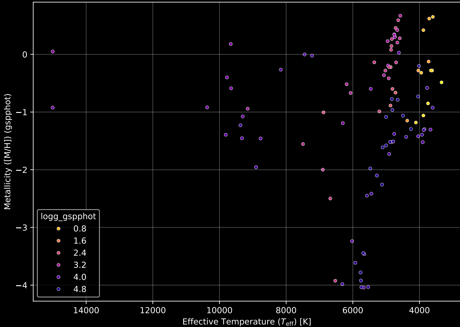
APOGEE DR17 Field: [004+02-O] Stellar Population Parameters (n= 104)
