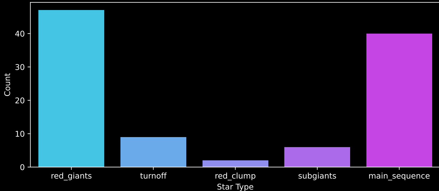
APOGEE DR17 Field: [004+02-O] Count plot of Star Type
