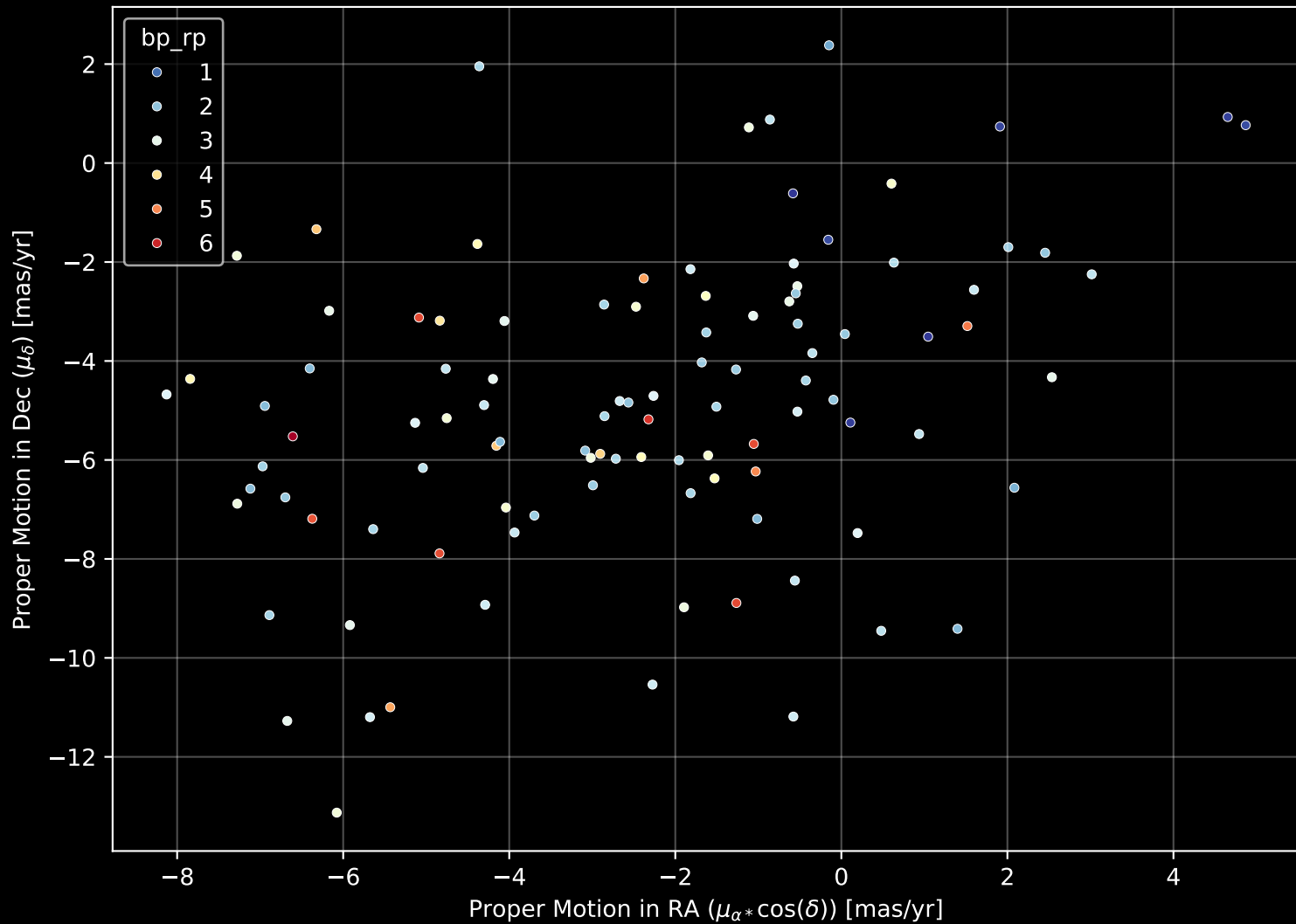
APOGEE DR17 Field: [004+02-O] Proper Motion Diagram (n= 104)
