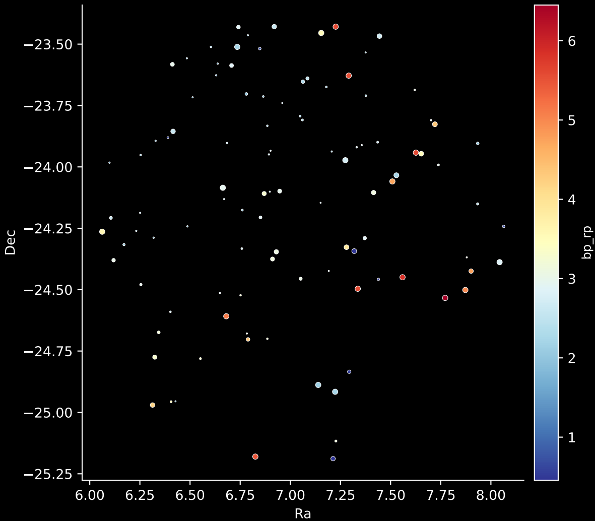
APOGEE DR17 Field: [004+02-O] Stars: 104
