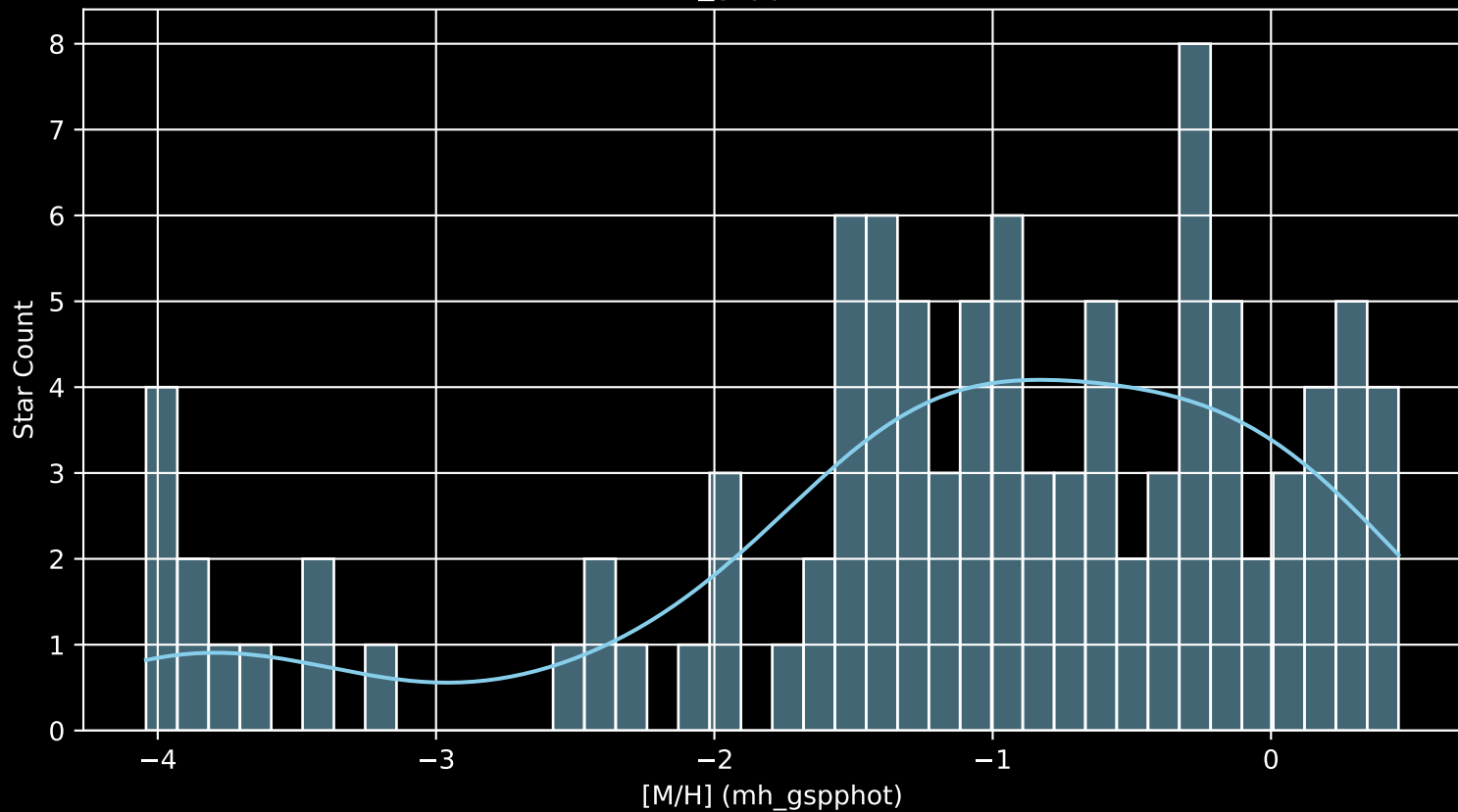
APOGEE DR17 Field: [004+02-O [M/H] (mh_gspphot) (n= 100)
