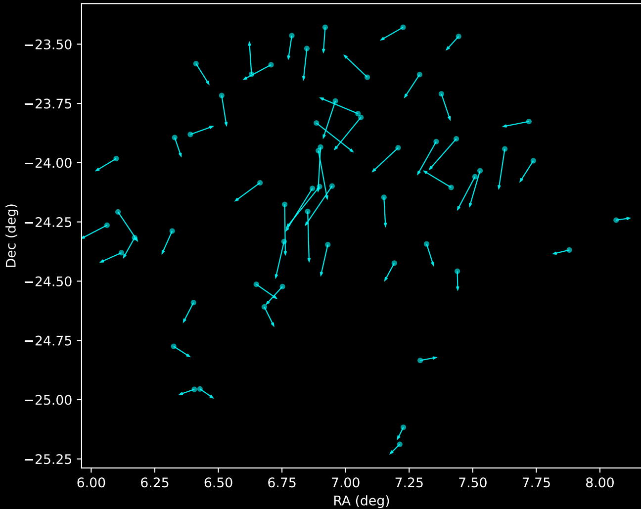
APOGEE DR17 Noise Stream Proper Motion Vectors (n=59)
